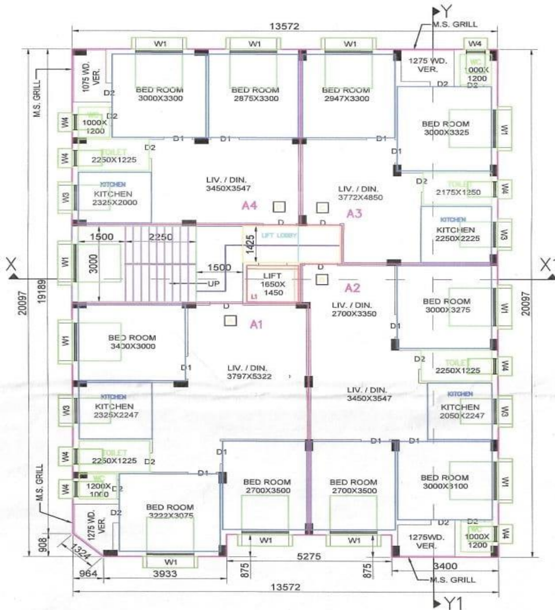
TYPICAL (1ST,2ND,3RD & 4TH) FLOOR PLAN BLOCK - A
